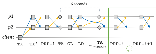
Fig. 6: The buggy execution triggering the liveness violation
